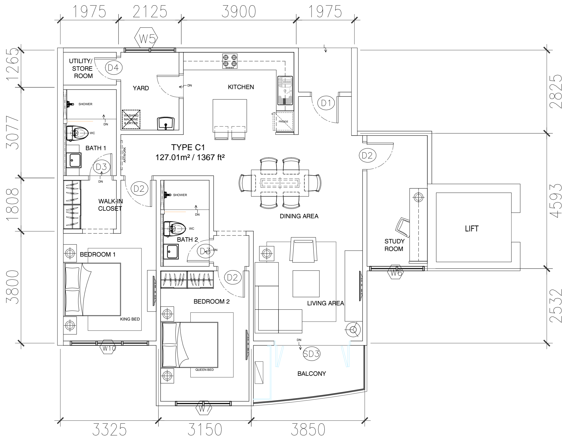
TYPICAL UNIT (TYPE C1) 127.1 sqm/1367 sqft SCALE = 1: 75
